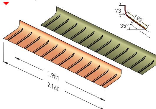
scossalina polivalente in HSP ed Ecotres
